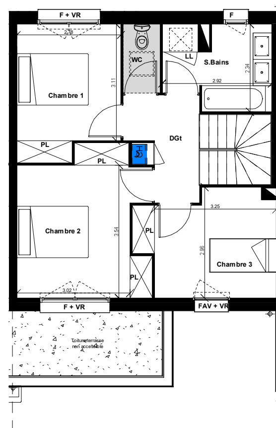
PLAN R+1
