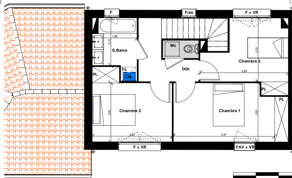
PLAN R+1
